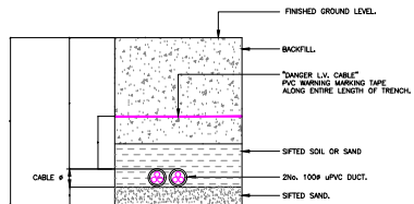
TYPICAL SECTION OF A BURIED L.V. CABLE SYSTEM (N.T.S.)
